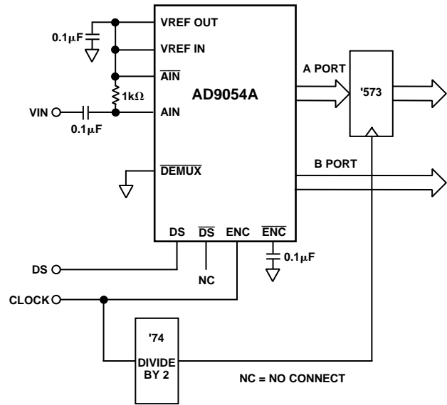
Figure 36. Dual Port Mode—Aligned Output Data
