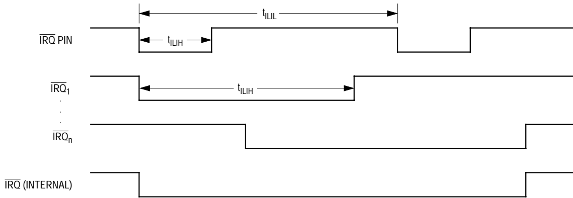
Figure 7. External Interrupt Timing
