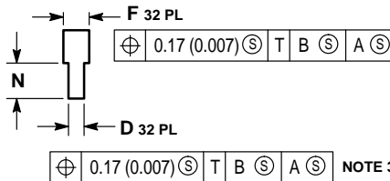
DETAIL Z
